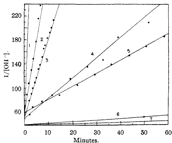
Fig. 1.—Bimolecular rate plots (numbers refer to compounds listed in Table I).
