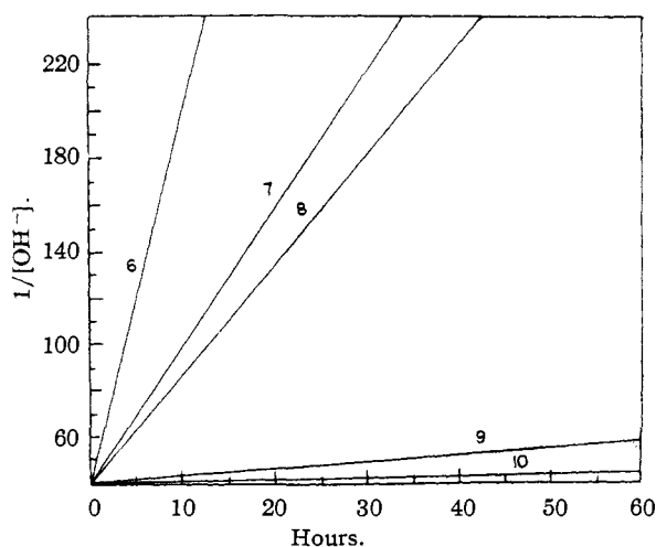
Fig. 2.—Bimolecular rate plots (numbers refer to compounds listed in Table I).
